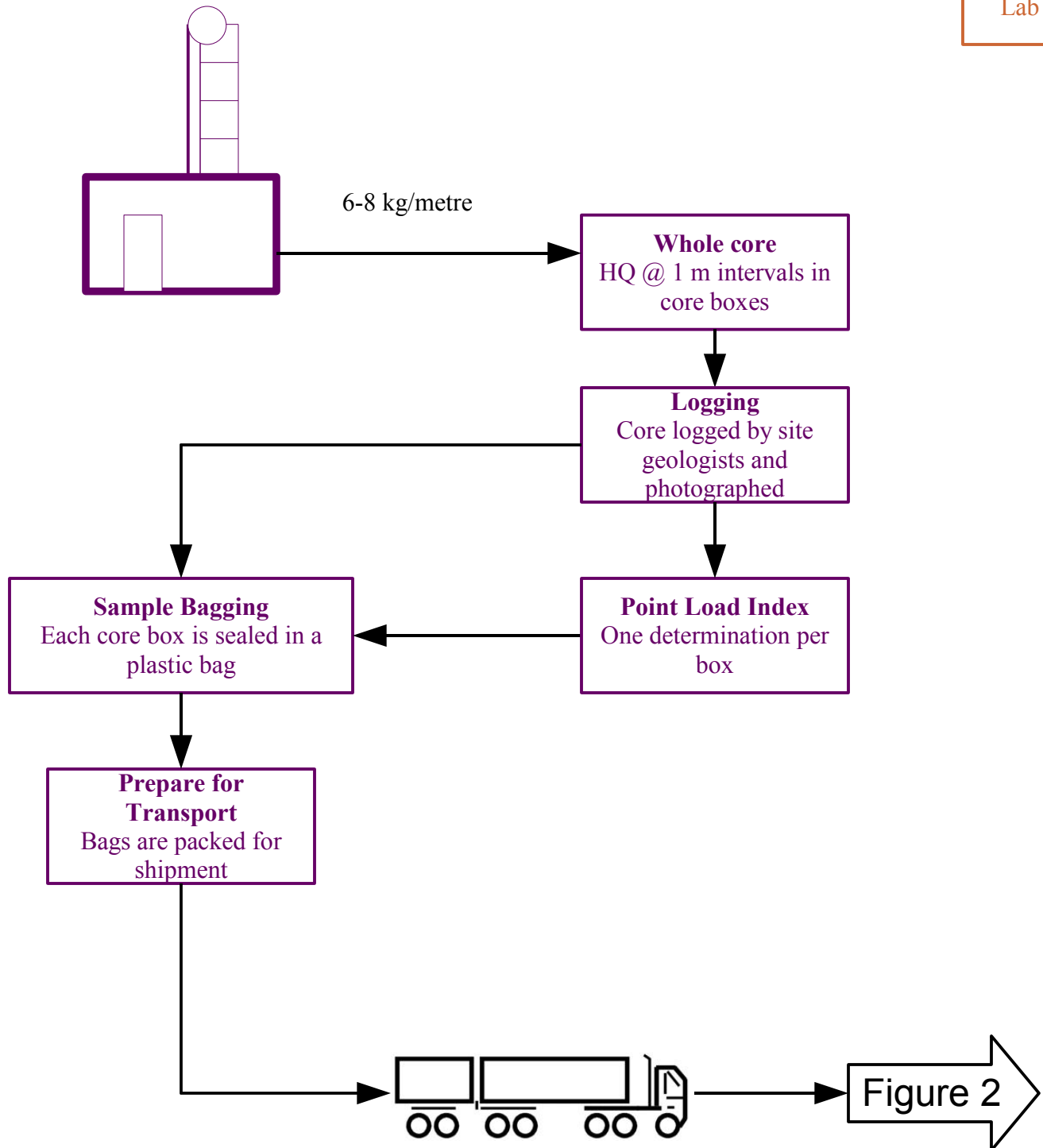
Figure 1: Composite Preparation Flowchart (whole HQ samples)
