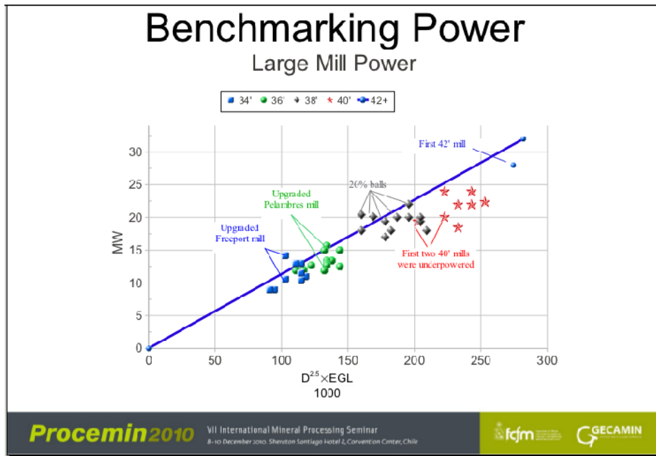
Figure 3: SAG Mill Motor Sizes Versus Function of Diameter (ft) and Effective Grinding Length (ft) 1
