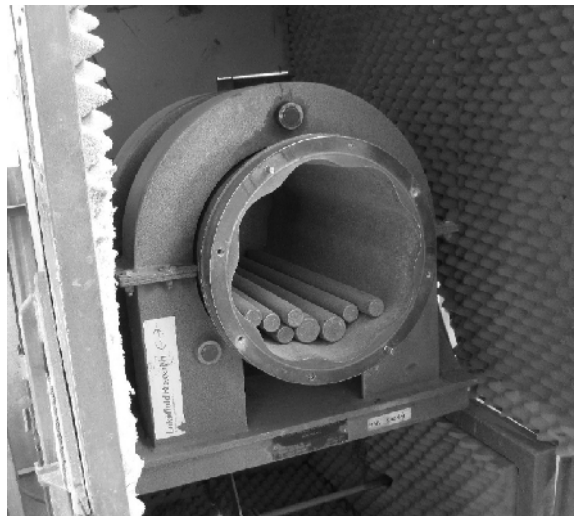
Figure 2: Rod mill for determining Bond rod mill work index
