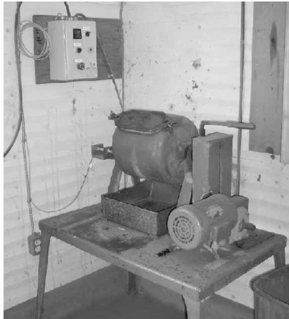
Figure 1: Ball mill for determining Bond ball mill work index
